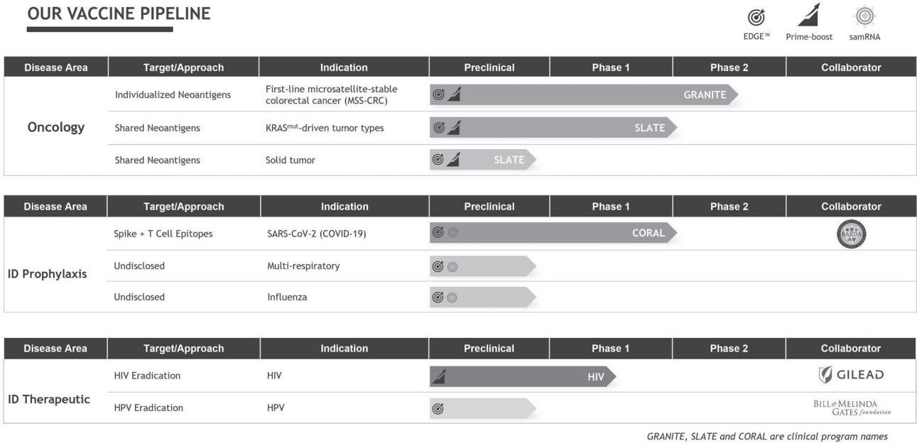
Figure 2. Our Pipeline
